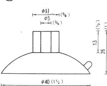
φ40立穴φ5 QT-40-5 2,000PCS
