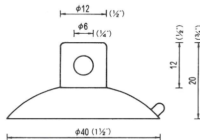
φ40横穴φ6 QY-40-6 2,500PCS
