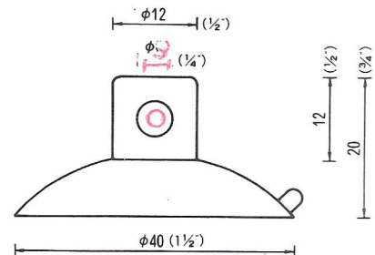
φ40横穴φ3 QY-40-3 2,500PCS
