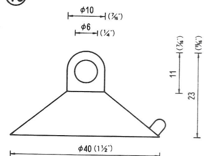
φ40横穴φ6肉厚 QY-40-6N 2,500PCS
