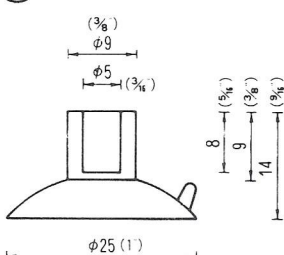
φ25立穴φ5 QT-25-5 5,000PCS
