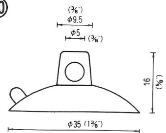
φ35横穴φ5シボ QY-35-5SB 2,500PCS
