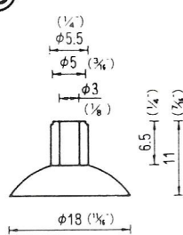
φ18立穴φ3 QT-18-3 5,000PCS
