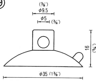
φ35横穴φ5 QY-35-5 2,500PCS
