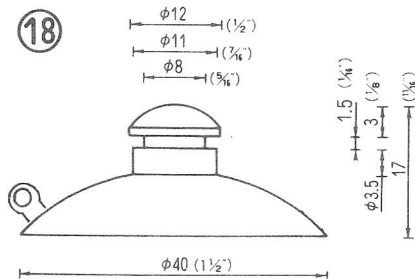
φ40横溝 QM-40 2,500PCS
