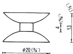
φ20 両面吸着盤 Both Type-20 QR-20 5,000PCS
