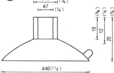
φ40立穴φ7 QT-40-7 2,000PCS
