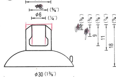
φ30立穴φ6 QT-30-6-ST 2,500PCS
