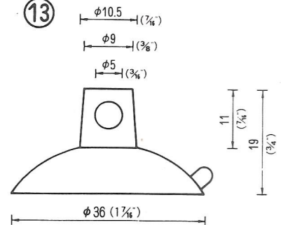
φ36横穴φ5 QY-36-5 2,500PCS
